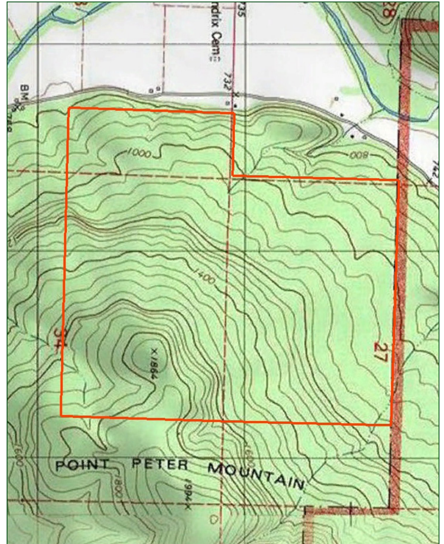
TOPOGRAPHY MAP FROM SURVEYOR
